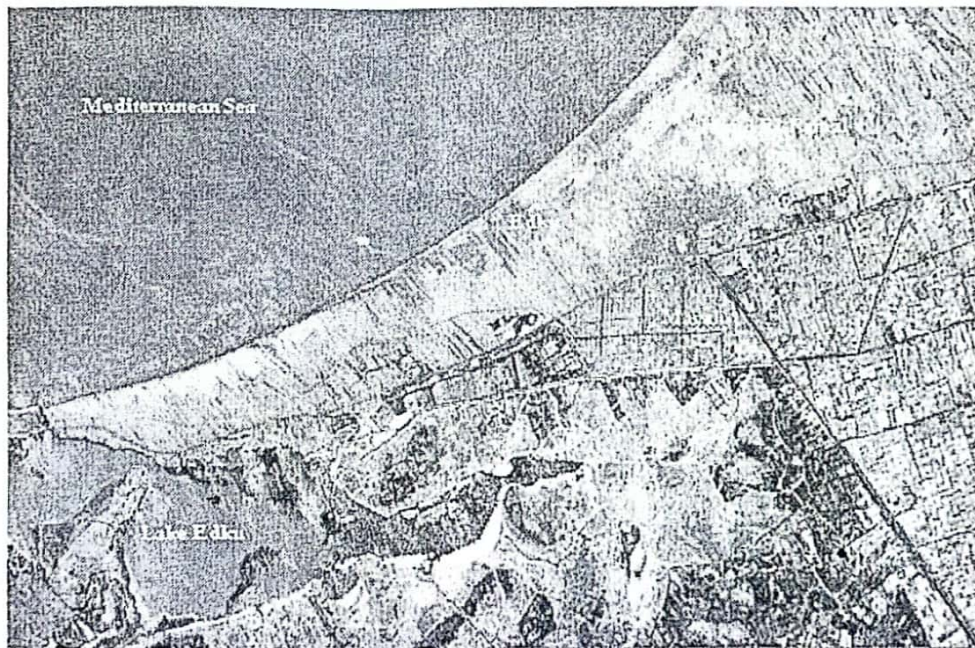
Figure (2). Basemap of Houd El-Remal subscene, scale: 1/125 000
