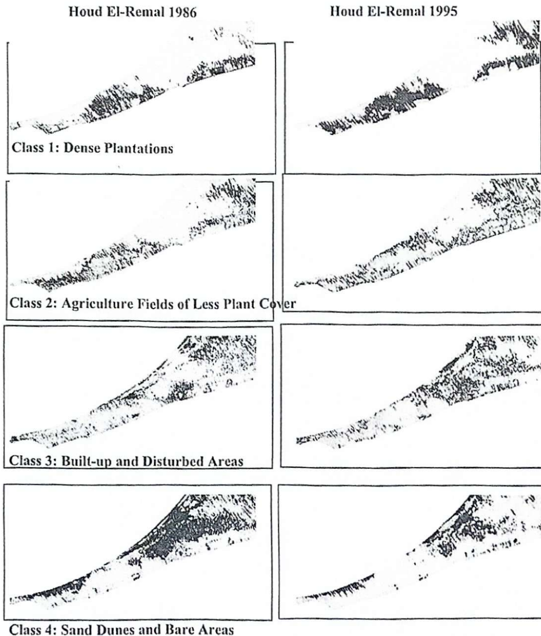
Figure (7). Unsupervised classification of Houd El-Remal area for 1986 scene (left column) and 1995 scene (right column), dark tone represents the spatial distribution of each class.
