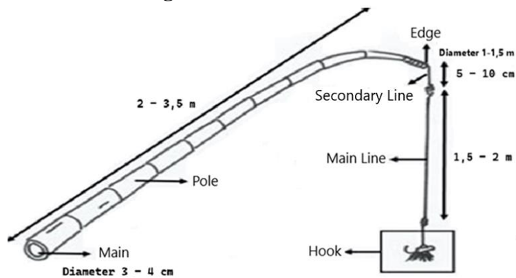
Fig. 4. Pole and line construction
