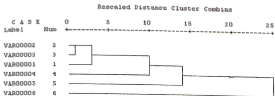
Fig. (2). Dendrogram of the micropropagated Balanites aegyptiaca using average linkage between plants.
