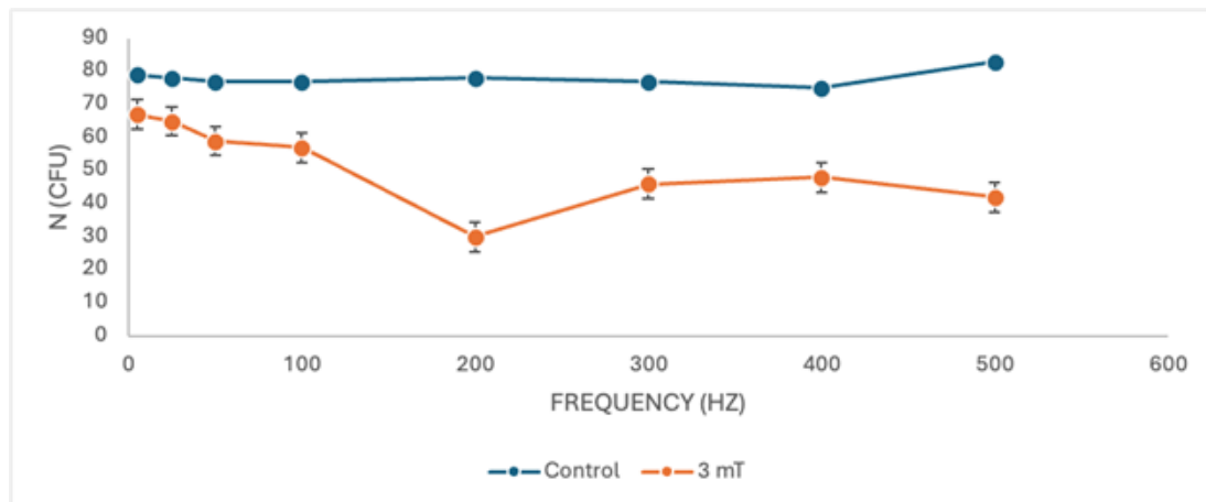
Figure 5: CFU count of E. coli after irradiation at 3 mT. Data is represented as means \pm SD from 3 different experiments.
