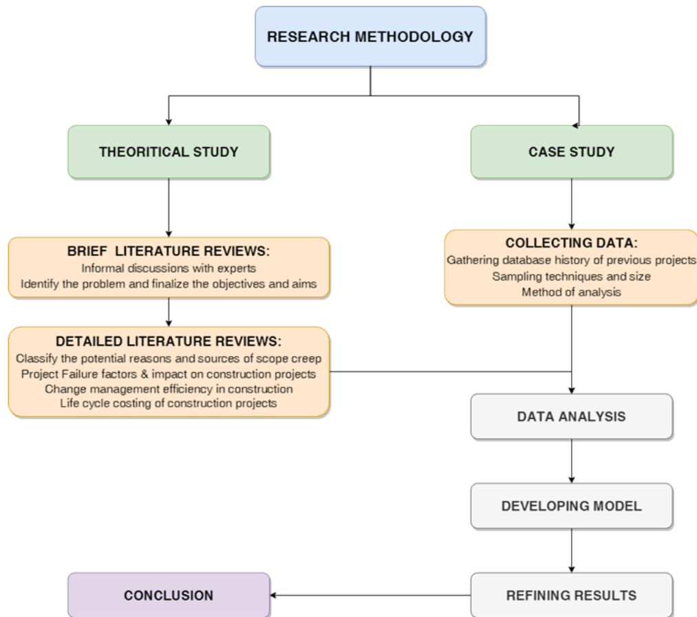
Figure 1: Research methodology
