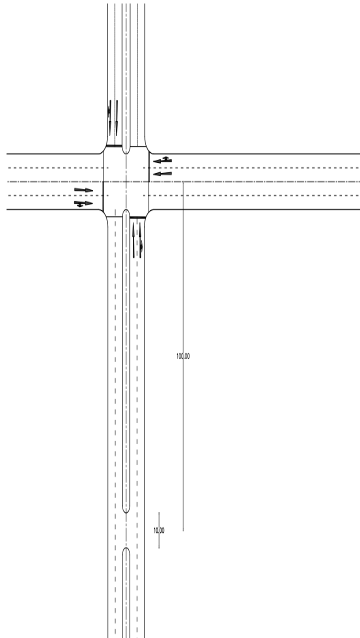
Figure 1. Geometric elements of the median U-turn intersection (MUT).
