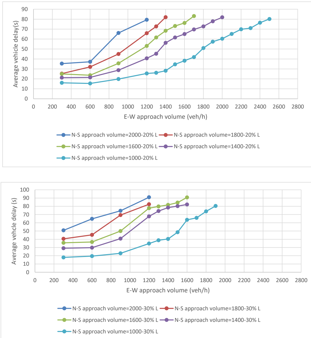
Figure 6. Average vehicle delay for the median U-turn intersection under unbalanced volume scenarios. (a) 20% LT (left-turn) and (b) 30% LT (left-turn).
