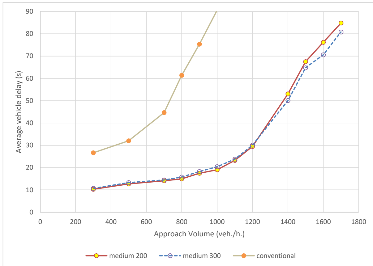
Figure 3. Delay comparison of the conventional, median U-turn (space distance 200), median U-turn (space distance 300).
