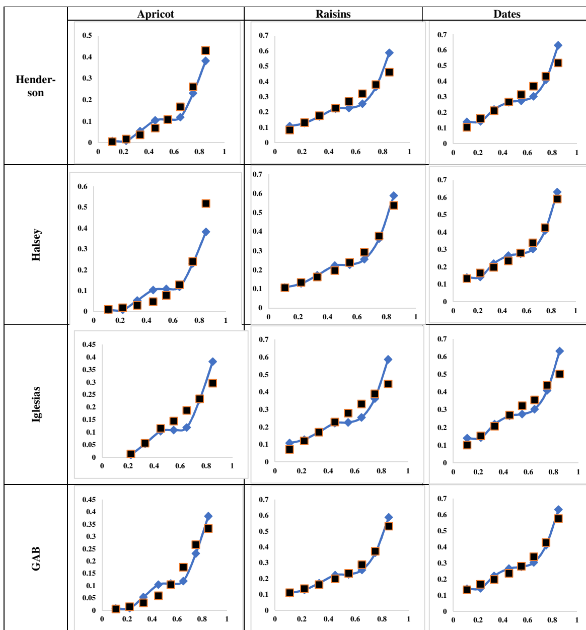
Figure (3): Comparison between experimental ( ) and calculated ( ) moisture content of dried fruits using different sorption isotherms equations. (Y axis : \text{g H}_2\text{O/g DM} and X axis : Water activity Value)
