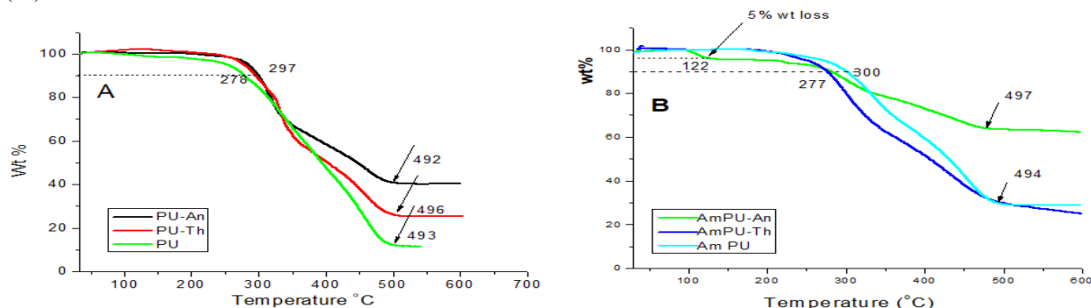
Figure 9: TGA thermograms of (A) PU and (B) AmPU before and after exposing to biodegradation.
