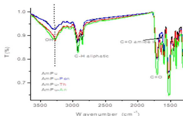
Figure 6: FTIR spectra of AmPU and biodegraded film samples.
