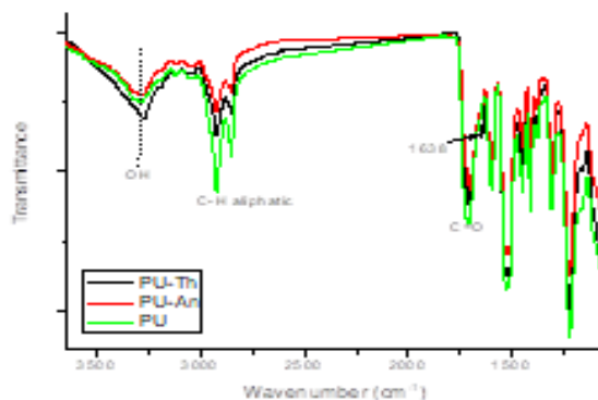
Figure 5: FTIR spectra of PU and biodegraded film samples
