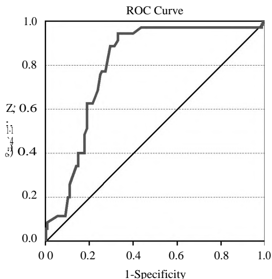
Fig. (4): ROC curve for Mean platelet volume.
