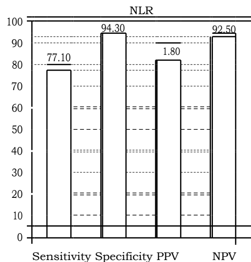
Fig. (3): Sensitivity, Specificity, PPV and NPV of NLR.
