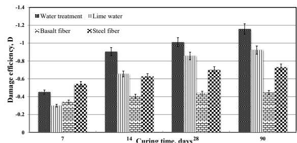
Fig. (3): Damage efficiency of 90 days alkali activated slag treated with various healing parameters.
