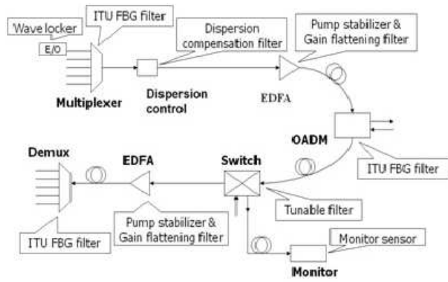
Fig. 5: FBG in OFC system
