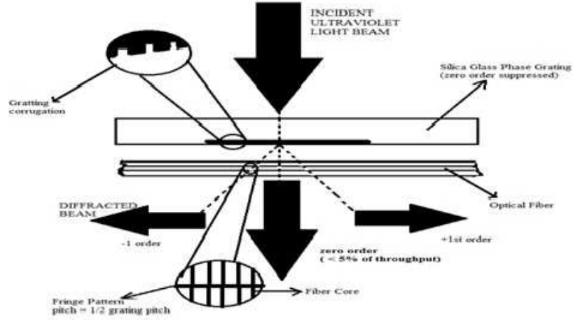
Fig. 3: Bragg grating fabrication apparatus based on a zero order null diffraction phase mask. The duty cycle of the phase mask is chosen to be 50% [7]
