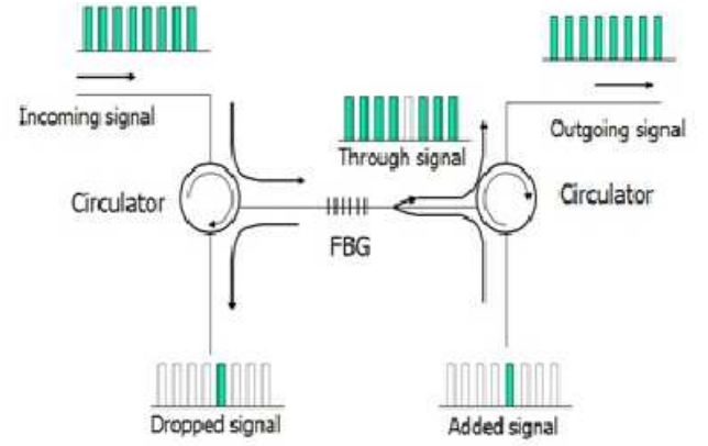
Fig. 7: OADM with the help of FBG[25]
