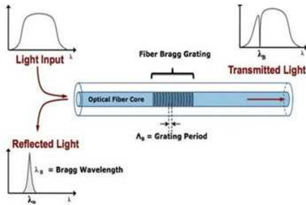
Fig. 9: Operation of the Fiber Bragg Grating sensor [32]
