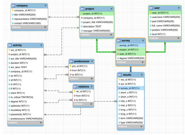
Fig. 1: Database structure.
