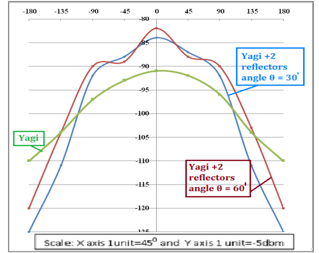
Fig. 3 Radiation patterns for Yagi with single reflector and multi reflector at different angles.
