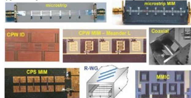
Fig.1. Typical metamaterial structures implementation [5].
