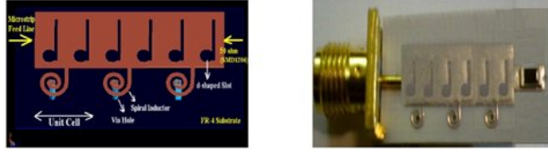
Simulated Prototype Fabricated Prototype.
