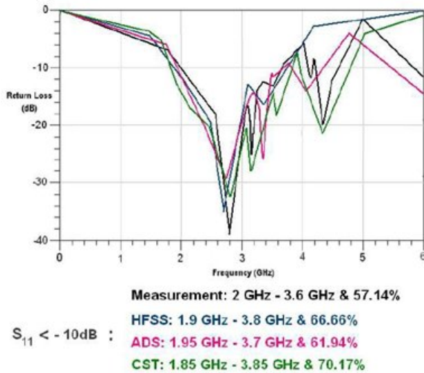
Fig.3. The simulated and measured return losses ( S_{11} < -10\text{dB} ) of the proposed d-shaped antenna. It should be emphasized that, the simulation return losses were obtained from High Frequency Structure Simulator (HFSS), Advance Design System (ADS), and CST Microwave Studio softwares.
