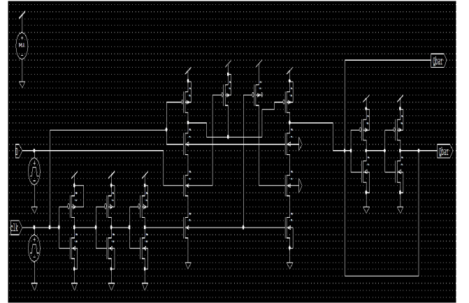
Fig. 8: Schematic of HLFF
