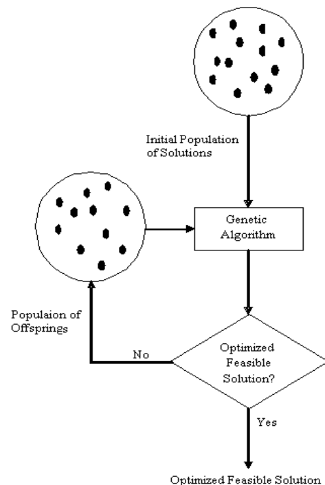
Figure 1 General Working Process of Genetic Algorithm GAs for Network Planning. These improved factors support a user for the selection of a Network with the desired parameters.
