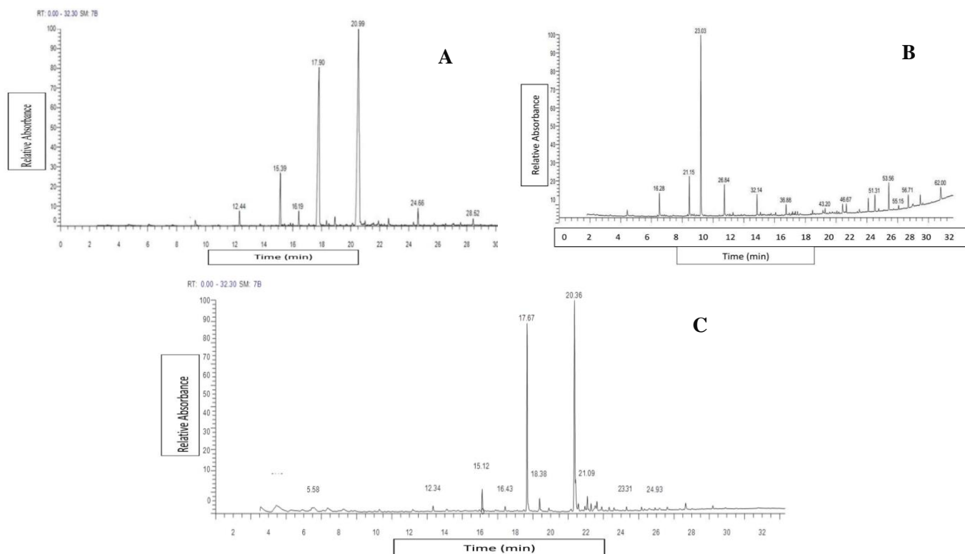
Figure 3. GC-MS chromatogram of extracts of C. longa . (A); aqueous extract: (B); ethanol extract: (C); ethyl acetate extract.
