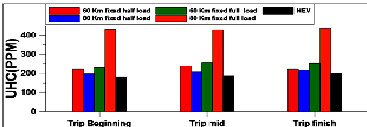
Fig. 17: UHC emission results
