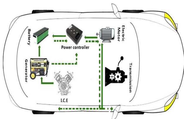
Fig. 6: Energy flow for PHEV
