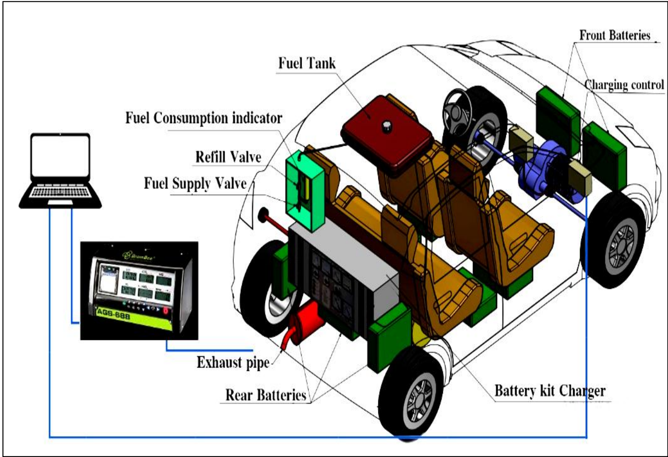
Fig. 8: Schematic diagram of the test system
