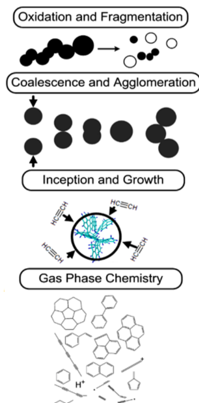
Figure 2. Schematic diagram of soot formation
