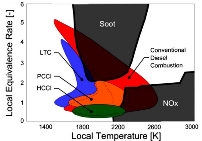
Figure 3. \Phi -T diagram of different combustion modes: CI, HCCI, and PCCI, on soot-NO x map
