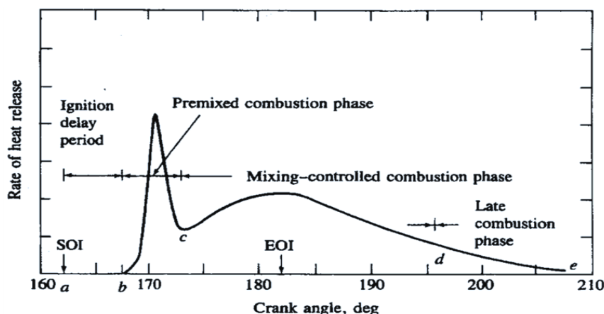
Figure 1. Typical heat release rate diagram identifying different diesel combustion phases
