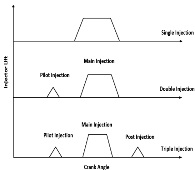
Figure 5. Injection profile for different injection strategies
