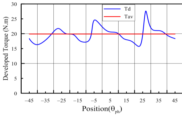
Figure 4: Developed torque with the position of rotor.
