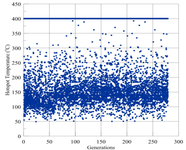
Figure 3: Hot-spot temperature of all design candidates.
