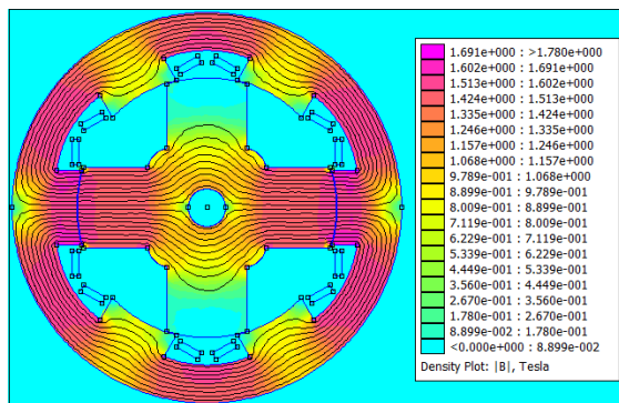
Figure 12: Flux distribution inside the optimal SRM in aligned position.
