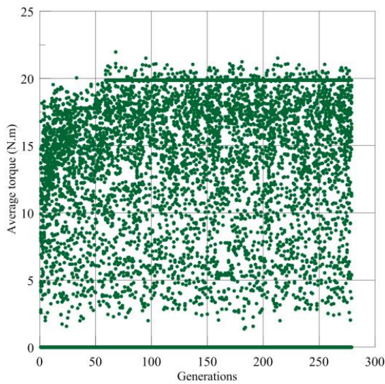
Figure 5: Average torque of all design candidates.
