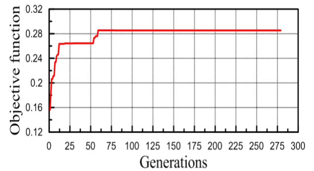
Figure 3: Total objective function's value of the optimal design with generations.
