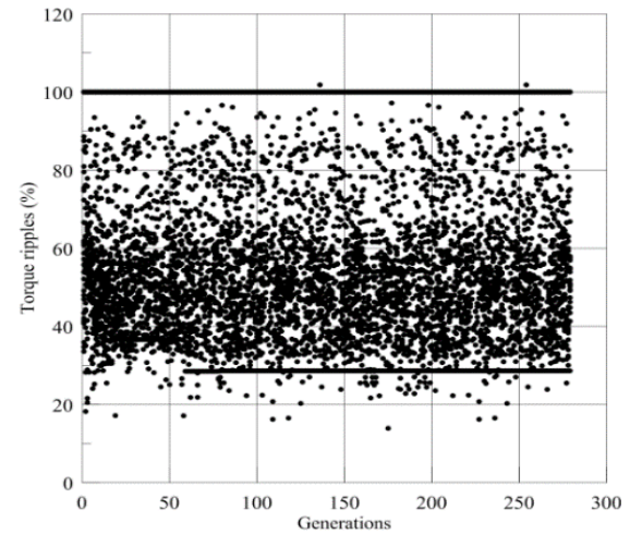
Figure 8: Torque ripples of all design candidates.
