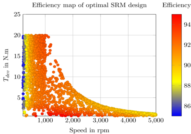
Figure 5: Efficiency map of the optimal design.
