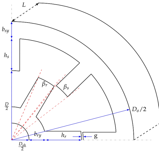
Figure 1: SRM design parameters considered in the optimization process.
