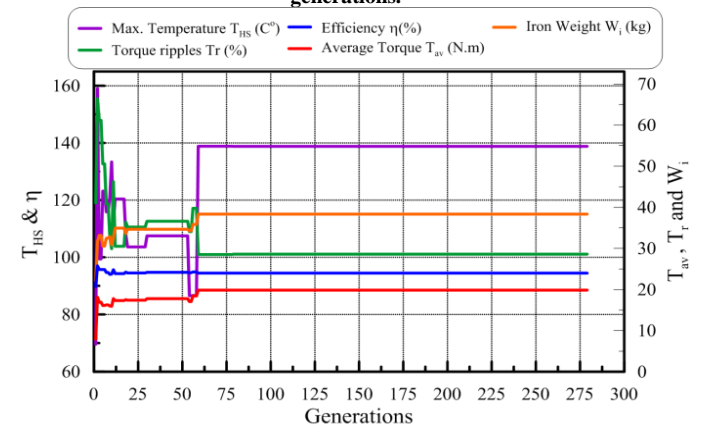
Figure 4: Characteristics values of the optimal design with generations.
