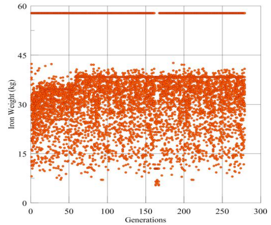
Figure 7: Iron weight of all design candidates.
