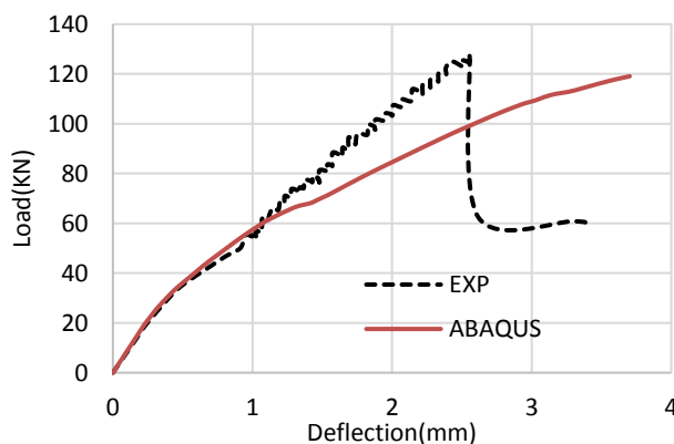
Fig. 14: Load-deflection curves for BI-1 specimen
