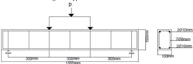
Fig. 3: Typical section of beam BIII-1.
