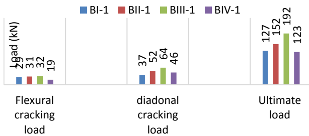
Fig. 6: Flexural cracking, critical shear crack and ultimate loads for the tested beams.
