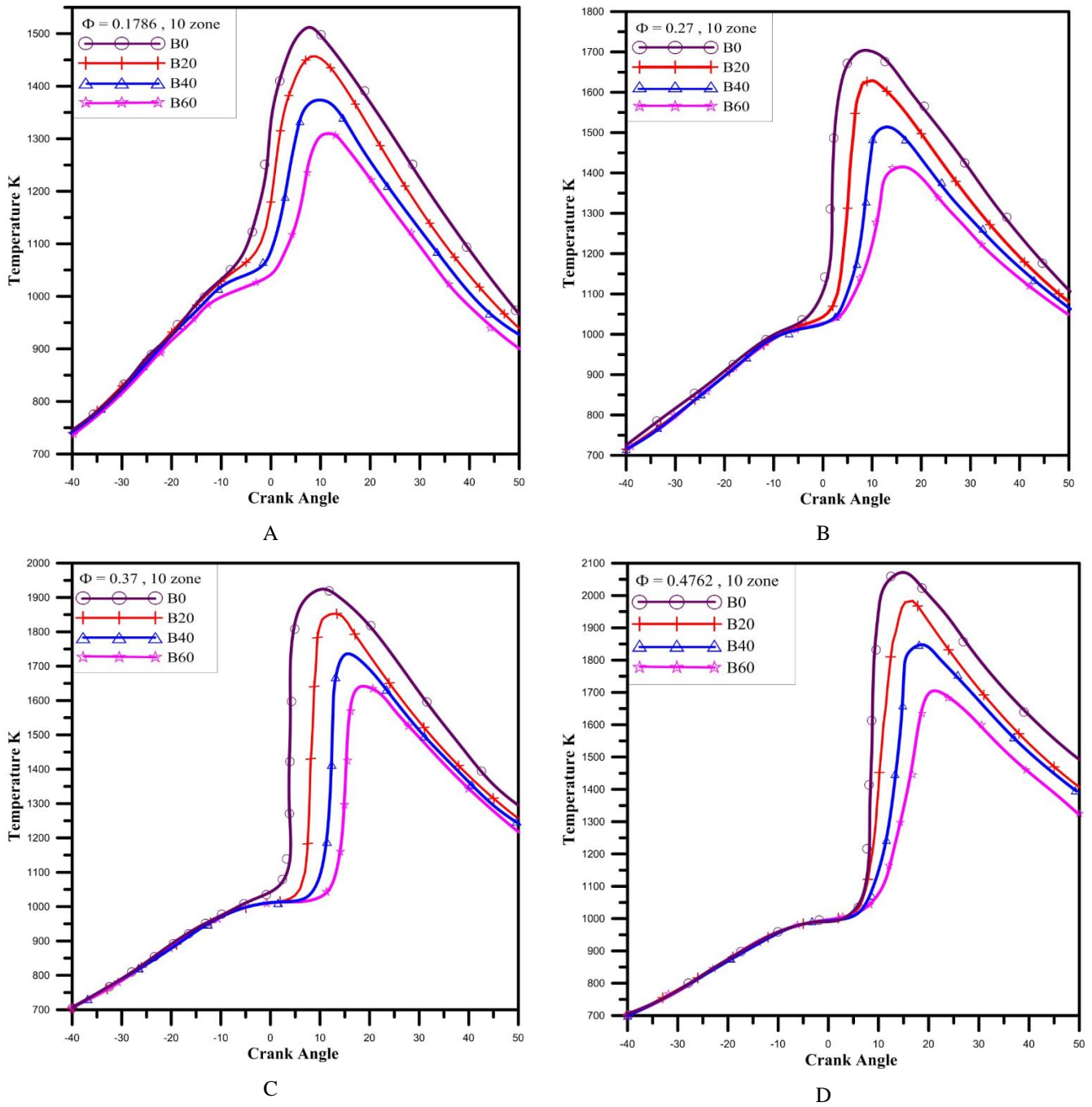
Fig. 6 Variation of the calculated Temperature for 10-zones model at different dose of Diesel/Biodiesel blends at different engine load, Cases of equivalence ratio represented in Table 3. However, the temperature histories of each zone inside the engine have been used to validate the assumption of zone configuration. The average temperature of multi-zones model was numerically calculated by using the multi-zone model.
