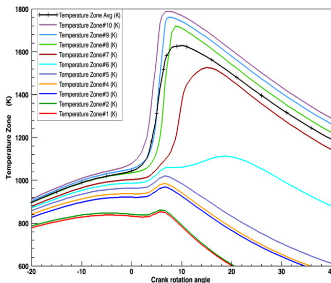
Fig. 2 The variation of the in-cylinder zones temperature for 10 zones model.
