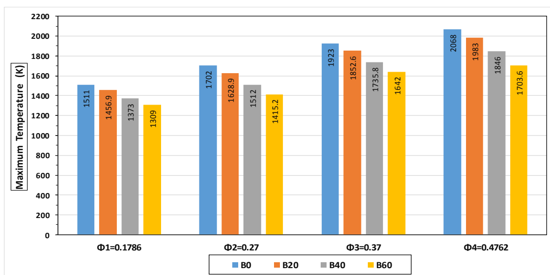
Fig. 9 Variation of the value of maximum temperature for 10-zones model at different dose of Diesel/Biodiesel blends at different engine load, Cases of equivalence ratio represented in Table 3
