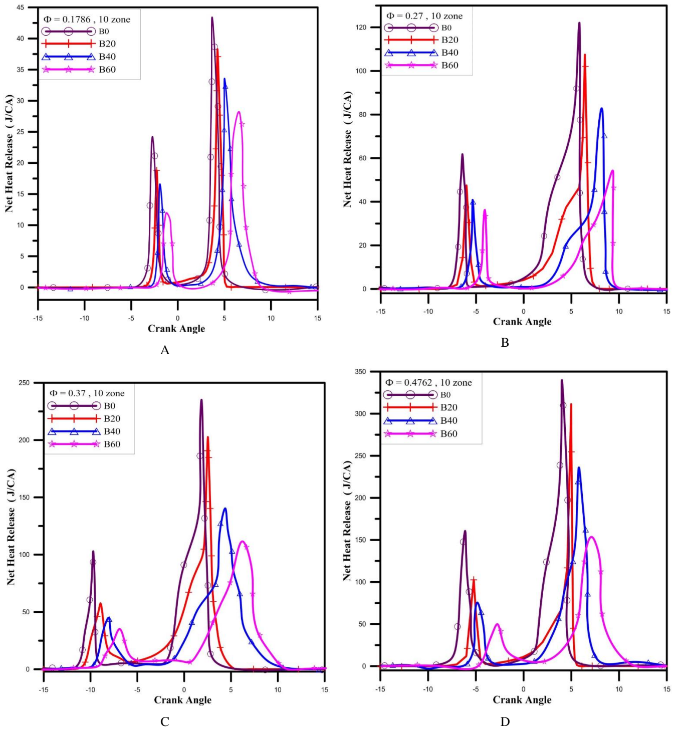
Fig. 7 Variation of the Net Heat Release for 10-zones model at different dose of Diesel/Biodiesel blends at different engine load, Cases of equivalence ratio represented in Table 3. However, the temperature histories of each zone inside the engine have been used to validate the assumption of zone configuration. The average temperature of multi-zones model was numerically calculated by using the multi-zone model.
