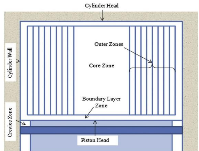
Fig. 1 Geometry of zones [12]
