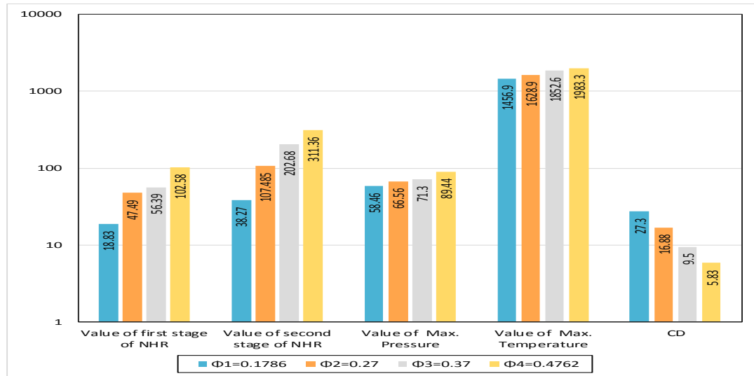
Fig. 3 variation of values of first stage of NHR, second stage of NHR, maximum pressure, maximum temperature and combustion duration for 10 zones model at cases of equivalence ratio.
