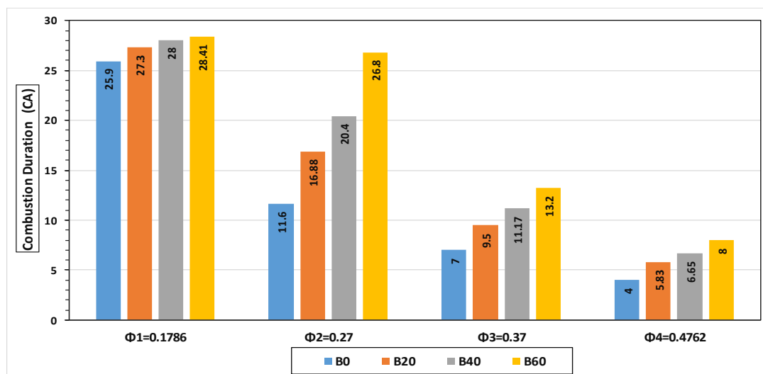
Fig. 10 Variation of the value of combustion duration for 10-zones model at different dose of Diesel/Biodiesel blends at different engine load, Cases of equivalence ratio represented in Table 3
