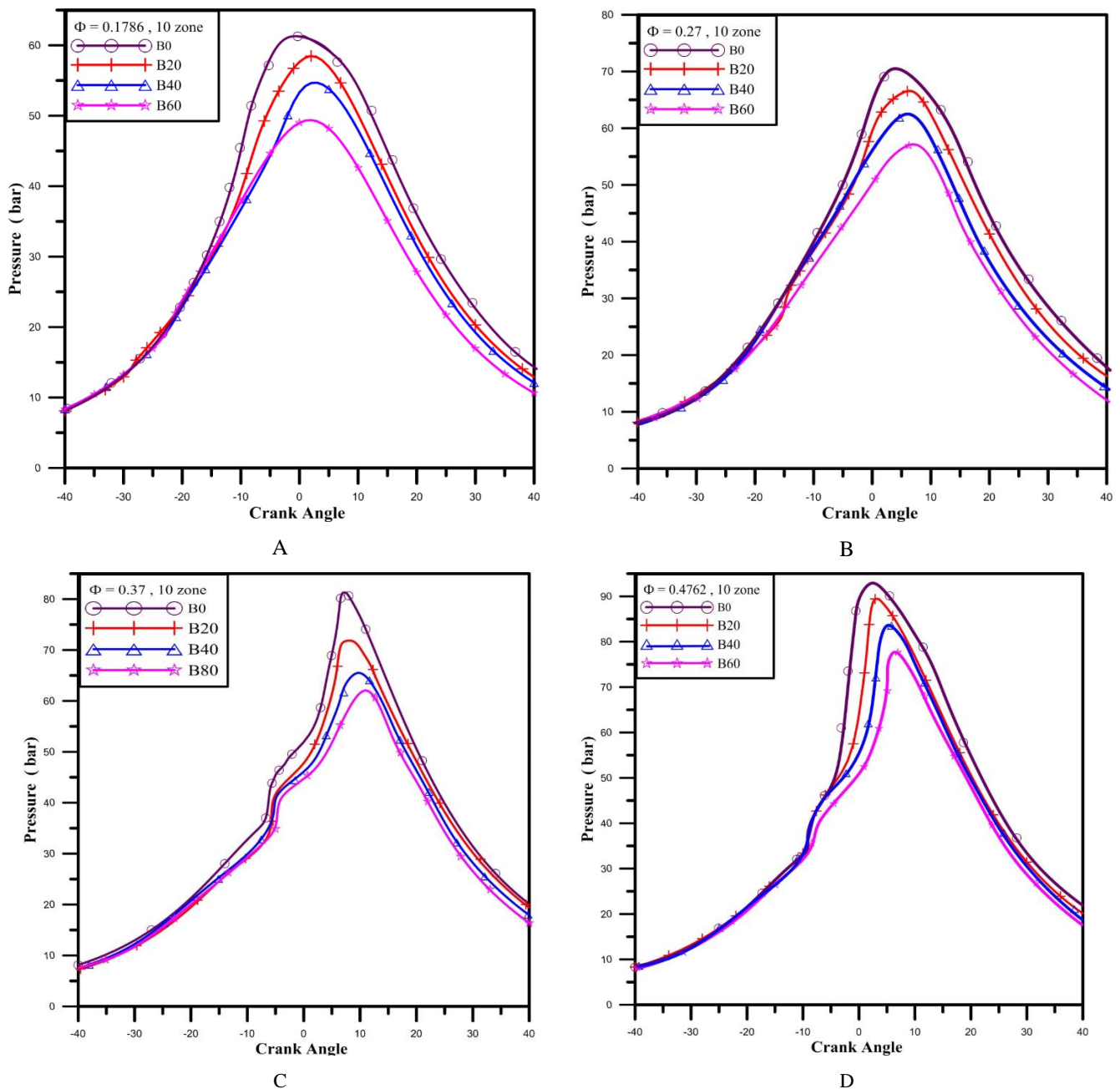
Fig. 5 Variation of the calculated pressure for 10-zones model at different dose of Diesel/Biodiesel blends at different engine load, Cases of equivalence ratio represented in Table 3. However, the temperature histories of each zone inside the engine have been used to validate the assumption of zone configuration. The average temperature of multi-zones model was numerically calculated by using the multi-zone model.
