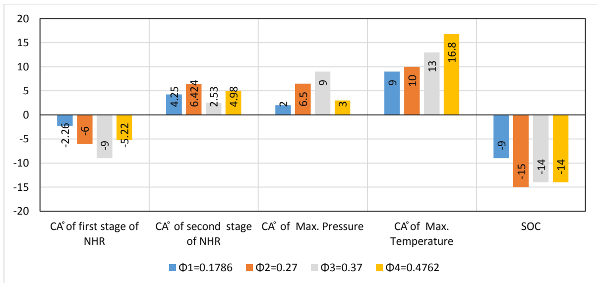
Fig. 4 variation of position of first stage of NHR, second stage of NHR, maximum pressure, maximum temperature and start of combustion for 10 zone model at cases of equivalence ratio.
