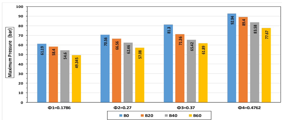
Fig. 8 Variation of the value of maximum pressure for 10-zones model at different dose of Diesel/Biodiesel blends at different engine load, Cases of equivalence ratio represented in Table 3
