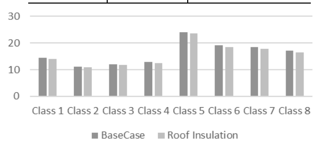
Fig. 18: Discomfort hours percentage- roof insulation
