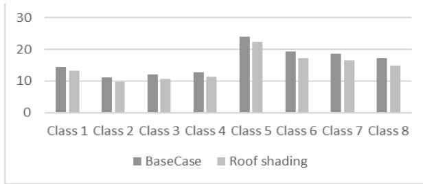
Fig. 19: Discomfort hours percentage- roof shading Roof shade installed parallel to the roof to minimize the direct solar radiation on the roof. The roof shade achieved great decrease in the discomfort hours as shown in table 20 and figure 19.
