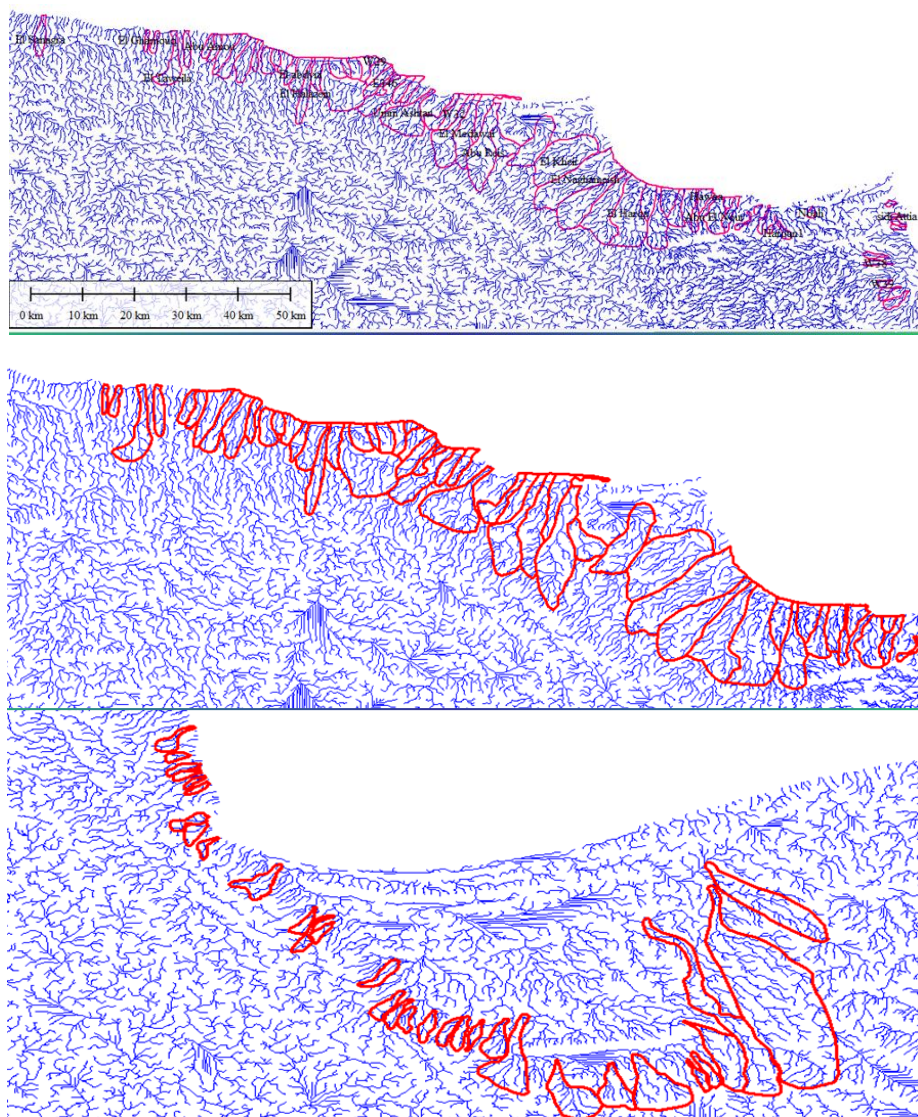
Fig.(4b) Drainage network and basin catchment area
