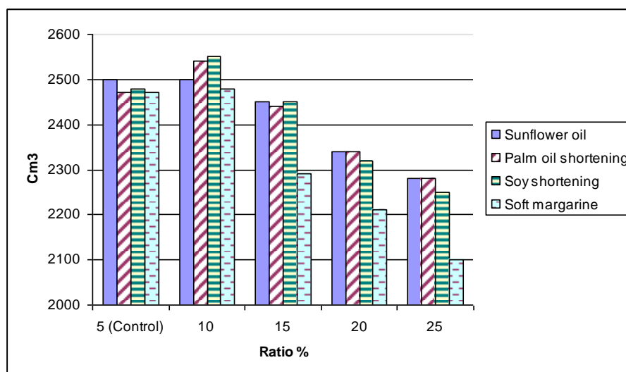
Figure (1): The Effect of different fatty matters and their adding ratios on bread volume
