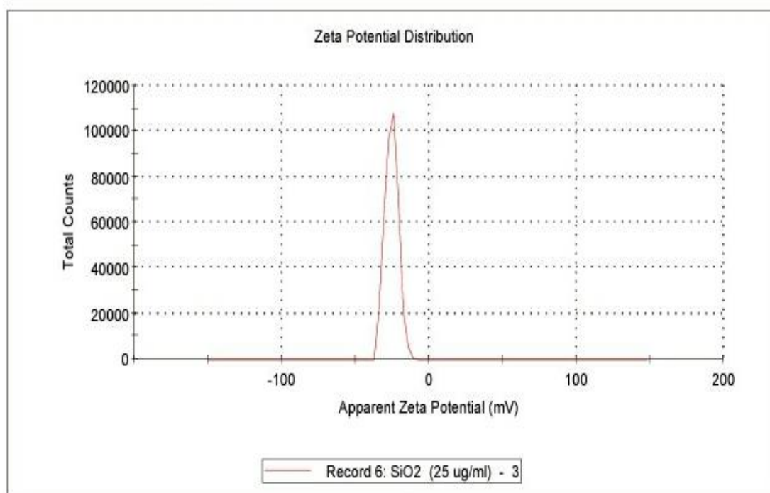
Fig 3 Zeta potential of green silicon dioxide nanoparticles.
