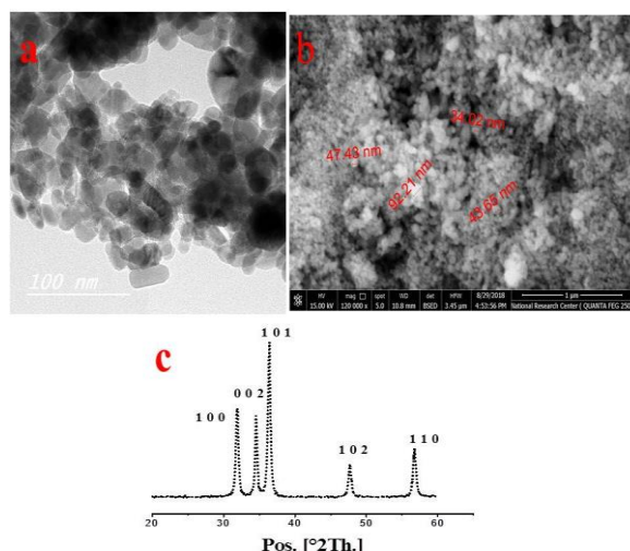
Fig. 1 The characterization of ZnO-NPs, TEM (a), SEM (b), and XRD pattern (c).
